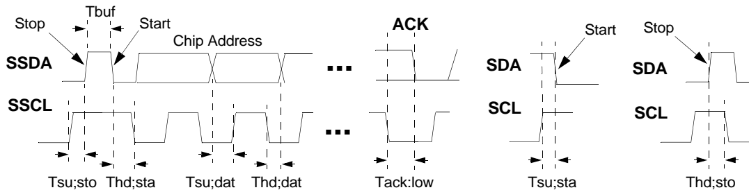
Figure 10. SSDA/SSCL Timing
